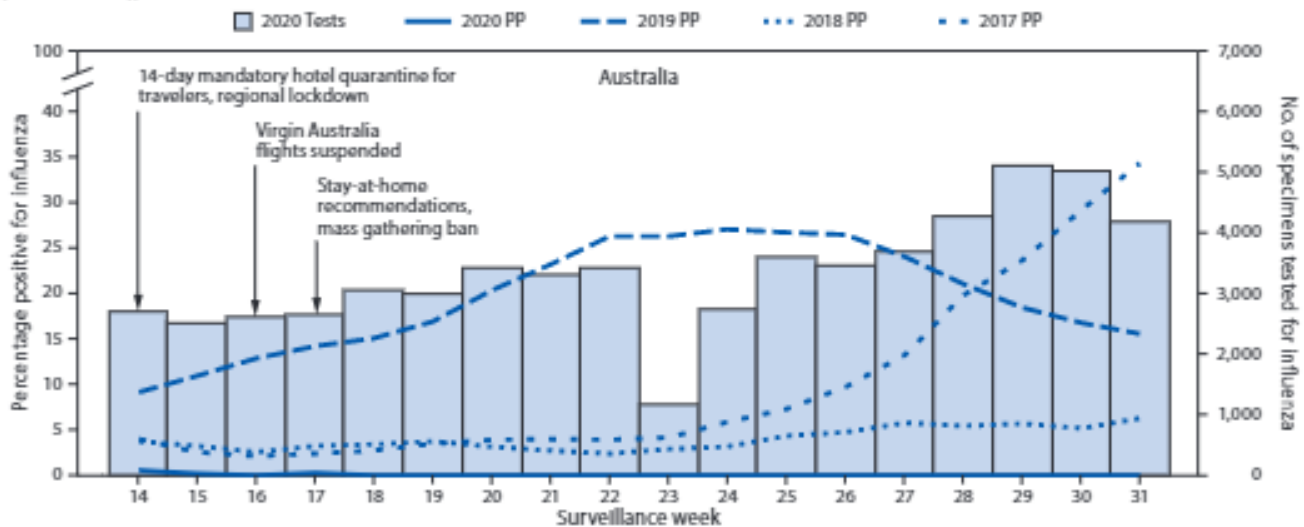
FIGURE 2. Number of specimens tested and percentage testing positive for influenza, by year — Australia, Chile, and South Africa, April–August (weeks 14–31), 2017–20
